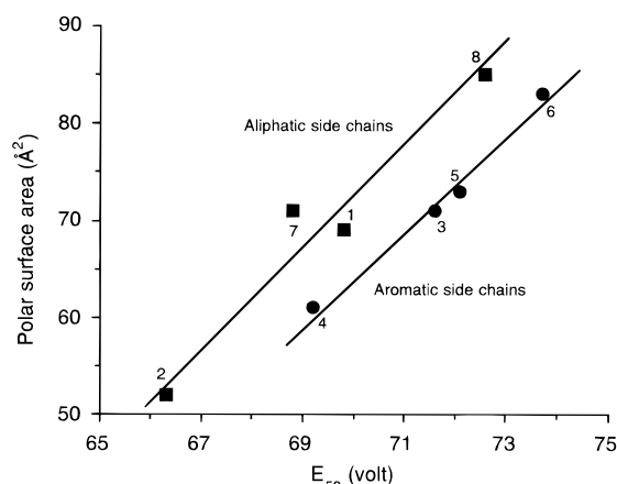
Figure 1. Plot of polar surface areas of the para -substituted benzene-sulfonamide inhibitors vs. the gas phase stabilities of the inhibitor-BCaII complexes, as measured by the amplitude of SORI-irradiation (E 50 ; Table 1). 6 For the same polar surface area, inhibitors with aromatic amino acid residues (circles) show stronger binding with BCaII in the gas phase than those with aliphatic side chains.
